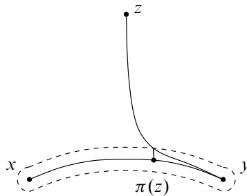
Figure 1.1: Handel–Mosher projection of a point z to the path from x to y
